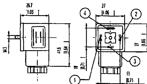
ELECTRIC CONNECTIONS SCHEME
