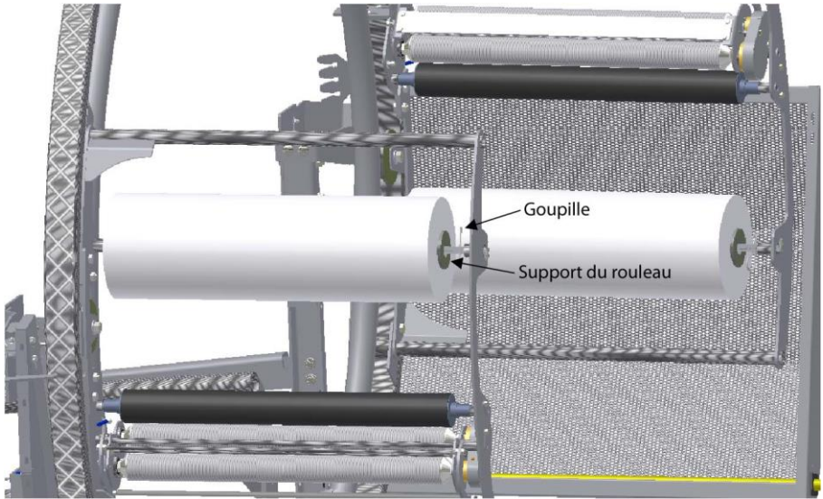
Figure 14 – Supports du rouleau de pellicule
