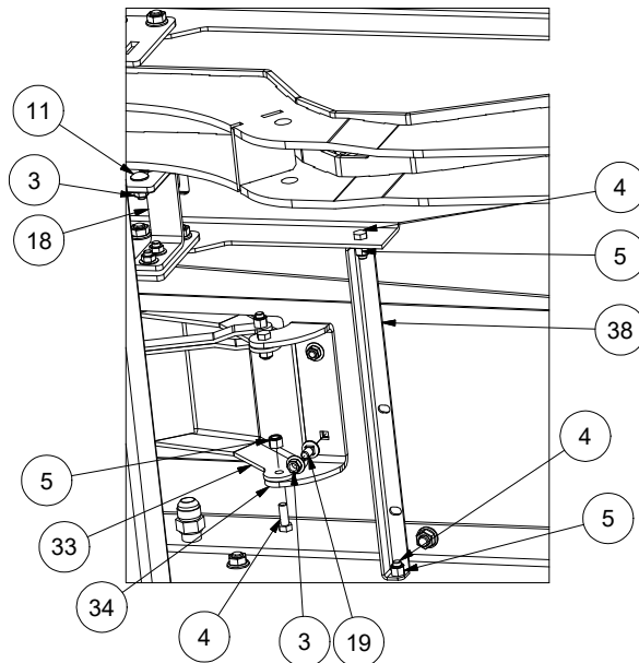
DETAIL A
