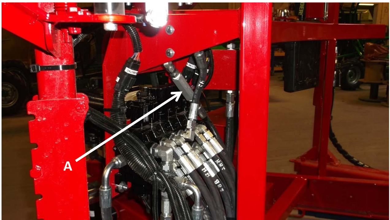
A- Check valve to be clean if cut & hold is opening very slowly.
