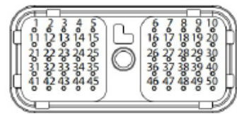
50-pin connector
